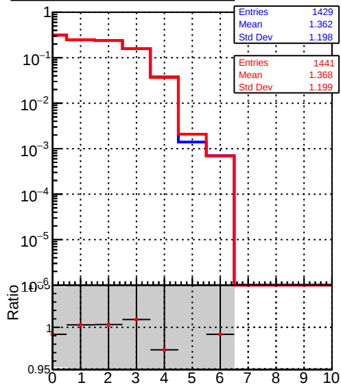
mean hit \eta Legend: DQM_CKF_TTbase (blue line), DQM_CKF_TT_retrainOldFiles125_v2_prelimWPM_epoch4 (red line)
