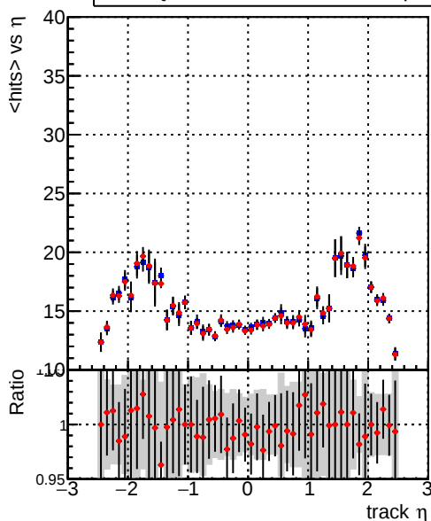
mean hit \eta Legend: DQM_CKF_TTbase (blue line), DQM_CKF_TT_retrainOldFiles125_v2_prelimWPM_epoch4 (red line)
