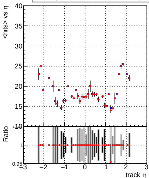
mean hits vs \eta Legend: DQM_CKF_TTbase (blue line with circles), DQM_CKF_TT_retrainOldFiles125_v2_prelimWPM_epoch4 (red line with circles)
