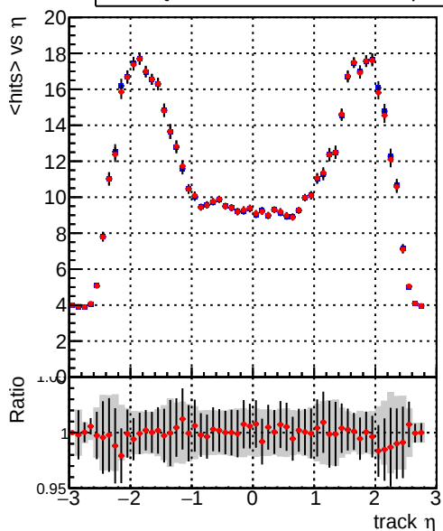
mean hit — DQM_CKF_TTbase — DQM_CKF_TT_retrainOldFiles125_v2_prelimWPM_epoch4
