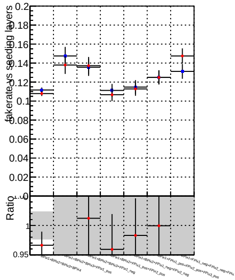
Fake rate vs. seeding layers —●— DQM CKF TTbase —●— DQM CKF TT_retrainOldFiles125_v2_prelimWPM_epoch4
