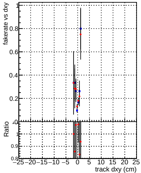
—●— DQM_CKF_TTbase —●— DQM_CKF_TT_retrainOldFiles125_v2_prelimWPM_epoch4
