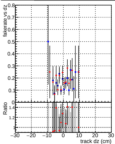
—●— DQM_CKF_TTbase —●— DQM_CKF_TT_retrainOldFiles125_v2_prelimWPM_epoch4
