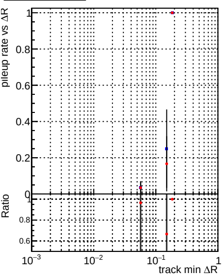
Legend: DQM_CKF_TTbase (blue), DQM_CKF_TT_retrainOldFiles125_v2_prelimWPM_epoch4 (red)
