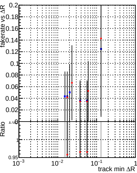
Legend: DQM_CKF_TTbase (blue), DQM_CKF_TT_retrainOldFiles125_v2_prelimWPM_epoch4 (red)
