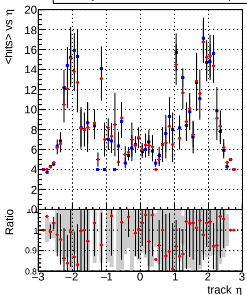
mean hit — DQM_CKF_TTbase — DQM_CKF_TT_retrainOldFiles125_v2_prelimWPM_epoch4
