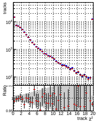
N of reco track vs. \chi^2 ● DOM_CKF_TTbase ● DOM_CKF_TT_retrainOldFiles125_v2_prelimWPM_epoch4
