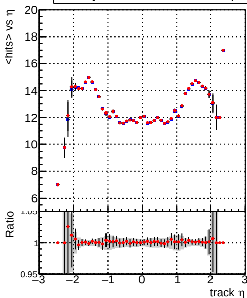
mean hits vs \eta — DQM_CKF_TTbase — DQM_CKF_TT_retrainOldFiles125_v2_prelimWPM_epoch4
