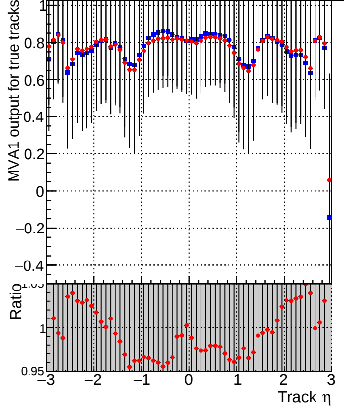
MVA1 of associated tracks (recoToSim) vs. track \eta Legend: ■ DQM_CKF_TTbase ◆ DQM_CKF_TT_retrainOldFiles125_v2_prelimWPM_epoch4
