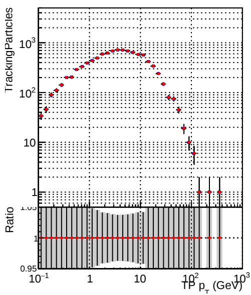
Legend: DQM_CKF_TTbase (blue line), DQM_CKF_TT_retrainOldFiles125_v2_prelimWPM_epoch4 (red line)
