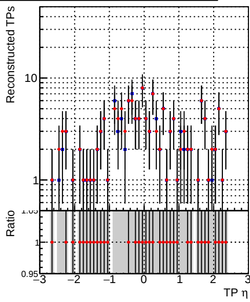
Legend: DQM_CKF_TTbase (blue line), DQM_CKF_TT_retrainOldFiles125_v2_prelimWPM_epoch4 (red line)
