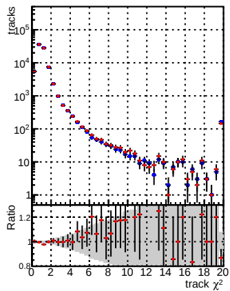
N of reco track vs. \chi^2 —●— DOM_CKF_TTbase —●— DOM_CKF_TT_retrainOldFiles25_v2_prelimWPM_epoch4
