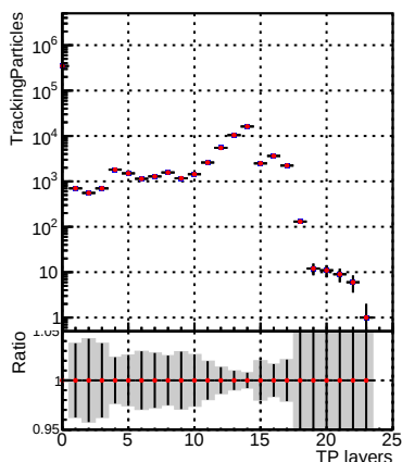
N of sim DQM_CKF_TTbase DQM_CKF_TT_retrainOldFiles125_v2_prelimWPM_epoch4
