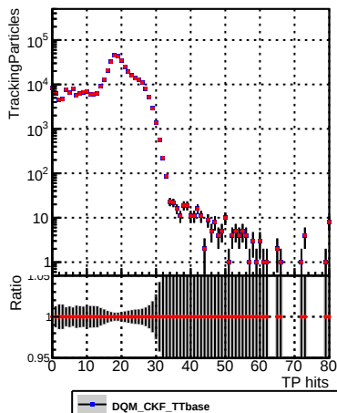
N of sim DQM_CKF_TTbase DQM_CKF_TT_retrainOldFiles125_v2_prelimWPM_epoch4
