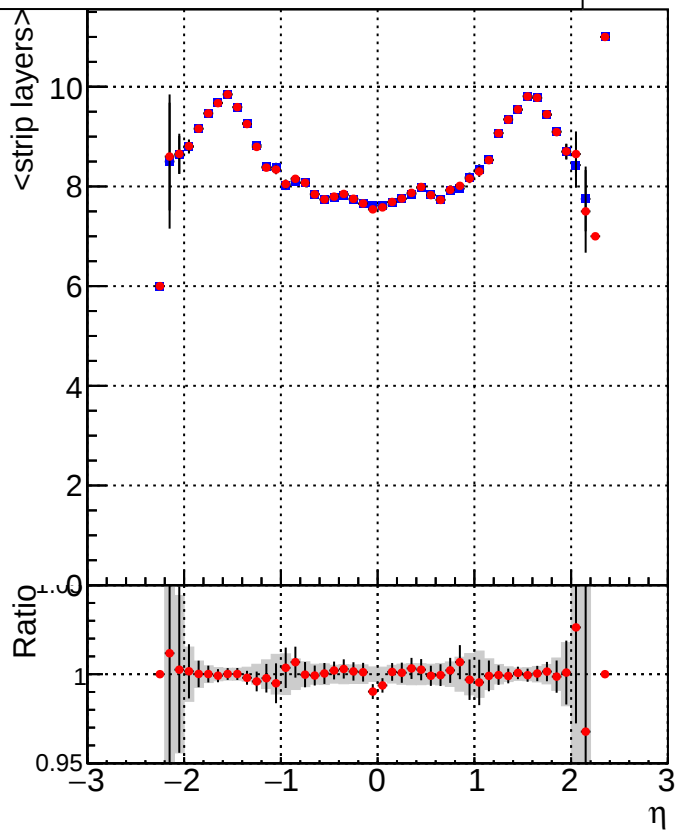
Legend: DQM_CKF_TTbase DQM_CKF_TT_retrainOldFiles125_v2_prelimWPM_epoch4
