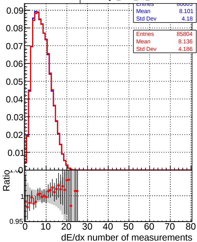
—■— DQM_CKF_TTbase —●— DQM_CKF_TT_retrainOldFiles125_v2_prelimWPM_epoch4
