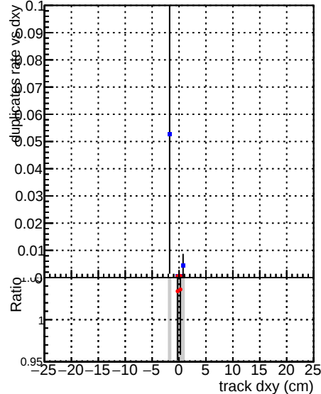
—■— DQM_CKF_TTbase —●— DQM_CKF_TT_retrainOldFiles125_v2_prelimWPM_epoch4
