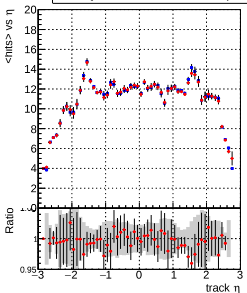
— DQM_CKF_TTbase — DQM_CKF_TT_retrainOldFiles125_v2_prelimWPM_epoch4 mean hits vs \eta
