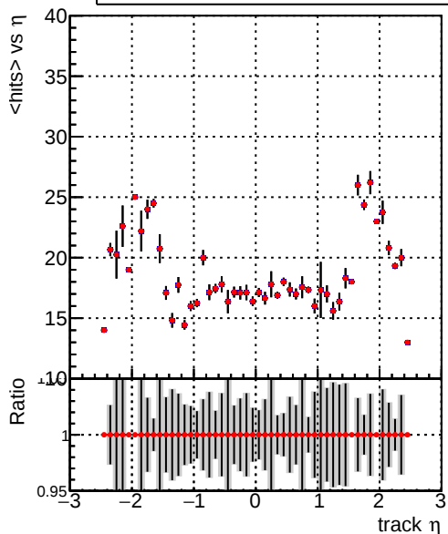
mean hits — DQM_CKF_TTbase — DQM_CKF_TT_retrainOldFiles125_v2_prelimWPM_epoch4
