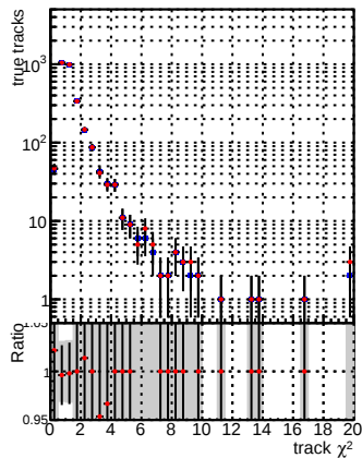
N of reco track vs. —●— DQM CKF TTbase —●— DQM CKF TT_retrainOldFiles125_v2_prelimWPM_epoch4
