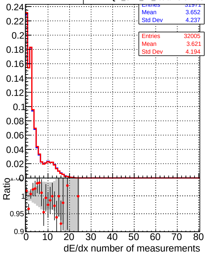
—■— DQM_CKF_TTbase —●— DQM_CKF_TT_retrainOldFiles125_v2_prelimWPM_epoch4
