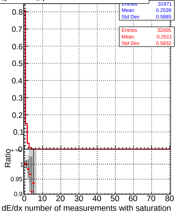
—■— DQM_CKF_TTbase —●— DQM_CKF_TT_retrainOldFiles125_v2_prelimWPM_epoch4
