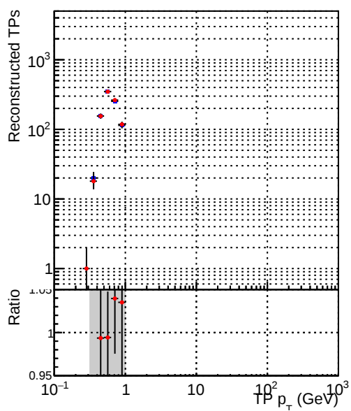
—•— DQM_CKF_TTbase —•— DQM_CKF_TT_retrainOldFiles125_v2_prelimWPM_epoch3
