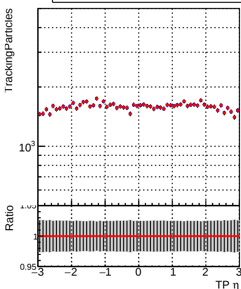
N of simulated tracks vs TP \eta — DQM_CKF_TTbase — DQM_CKF_TT_retrainOldFiles125_v2_prelimWPM_epoch3
