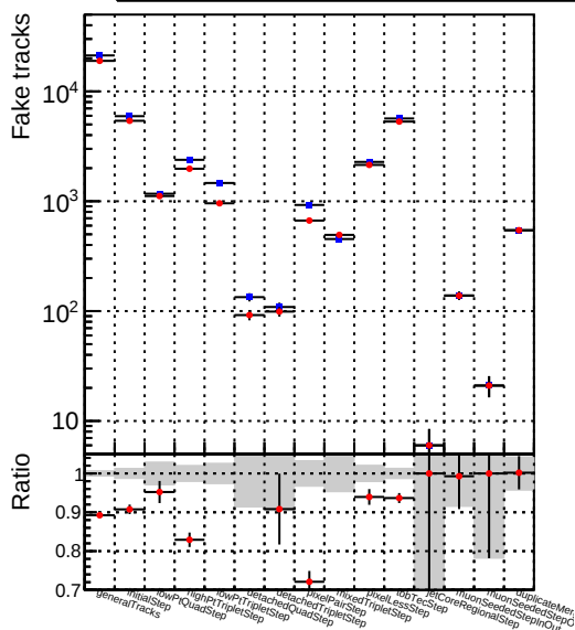
Number —●— DQM_CKF_TT_retrainOldFiles125_v2_prelimWPM_epoch3
