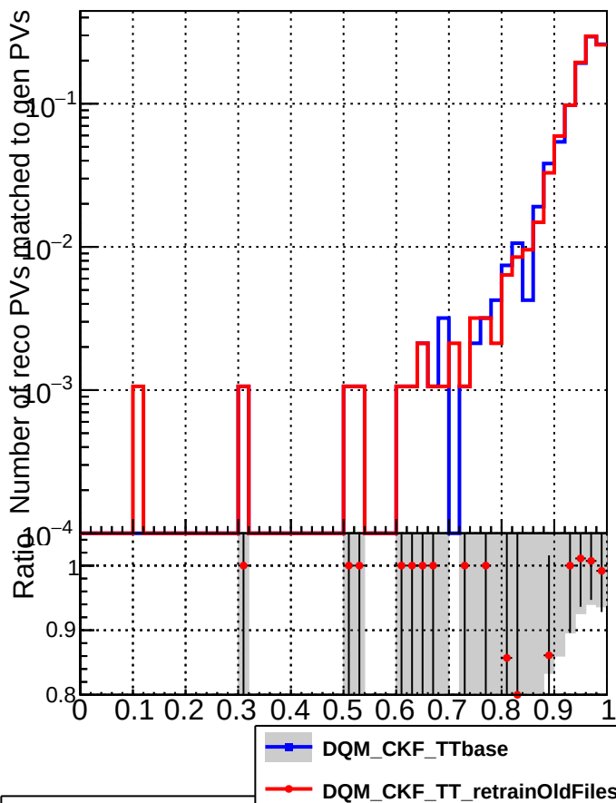
RecoPVAssoc2GenPVmatched_missing
