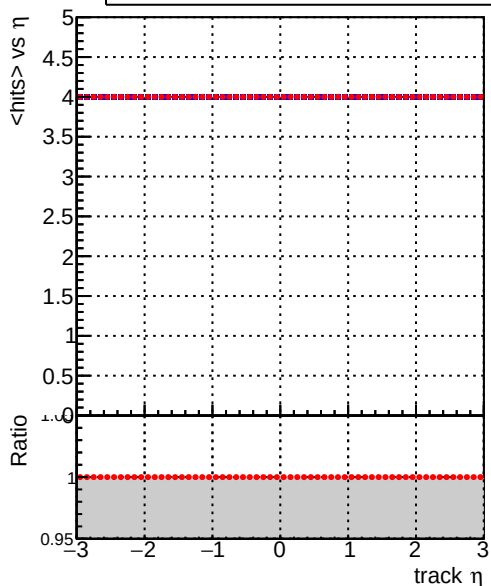
mean hits — DQM_CKF_TTbase — DQM_CKF_TT_retrainOldFiles125_v2_prelimWPM_epoch3
