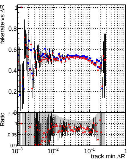
—•— DQM_CKF_TTbase —•— DQM_CKF_TT_retrainOldFiles125_v2_prelimWPM_epoch3
