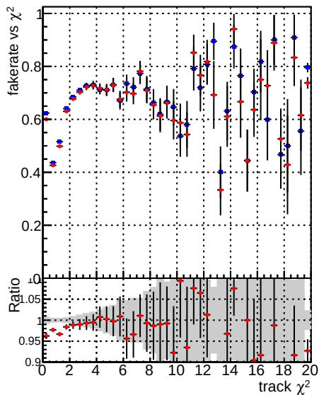
Fake rate vs. \chi^2 Legend: DQM CKF TTbase (blue) DQM CKF TT_retrainOldFiles125_v2_prelimWPM_epoch3 (red)
