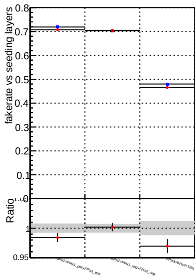
Fake rate vs. —●— DQM_CKF_TTbase —●— DQM_CKF_TT_retrainOldFiles125_v2_prelimWPM_epoch3
