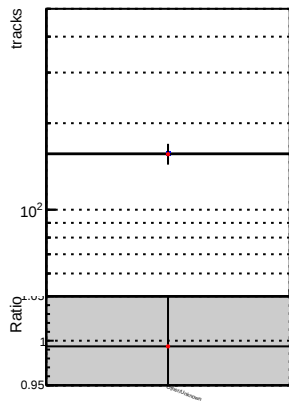
N of reco track vs. \chi^2 —•— DQM_CKF_TTbase —•— DQM_CKF_TT_retrainOldFiles125_v2_prelimWPM_epoch3
