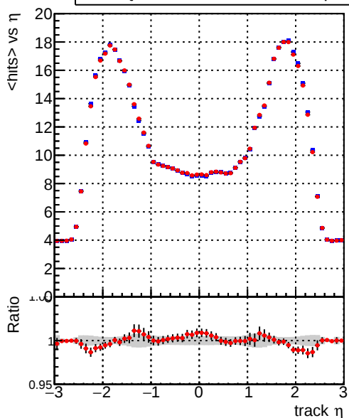
mean hits vs \eta — DQM_CKF_TTbase — DQM_CKF_TT_retrainOldFiles125_v2_prelimWPM_epoch3
