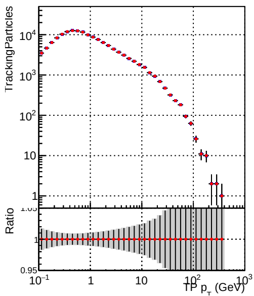
—•— DQM_CKF_TTbase —•— DQM_CKF_TT_retrainOldFiles125_v2_prelimWPM_epoch3
