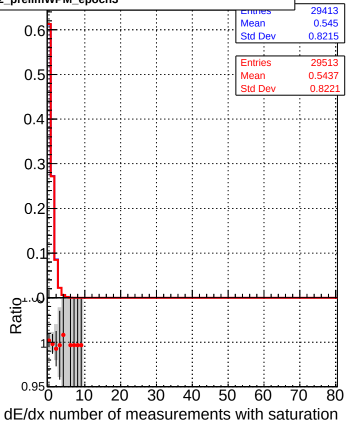
—■— DQM_CKF_TTbase —●— DQM_CKF_TT_retrainOldFiles125_v2_prelimWPM_epoch3
