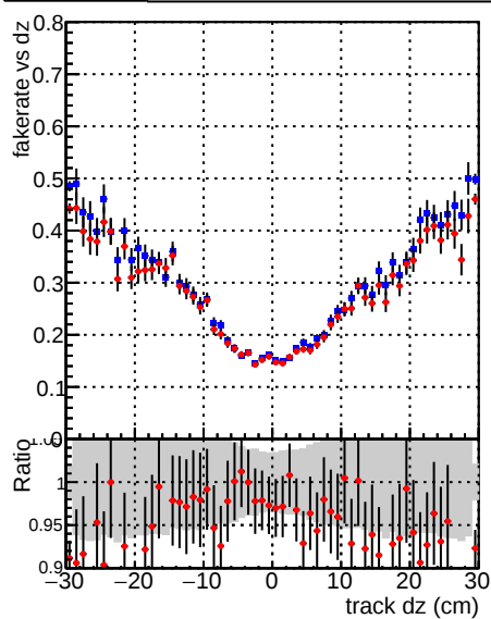
—●— DQM_CKF_TTbase —●— DQM_CKF_TT_retrainOldFiles125_v2_prelimWPM_epoch3
