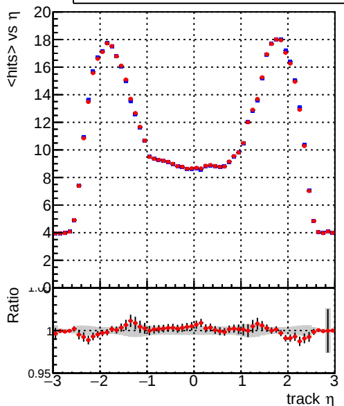
— DQM_CKF_TTbase — DQM_CKF_TT_retrainOldFiles125_v2_prelimWPM_epoch3 mean hits vs \eta
