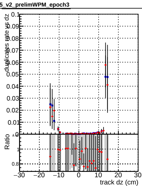
—●— DQM_CKF_TTbase —●— DQM_CKF_TT_retrainOldFiles125_v2_prelimWPM_epoch3
