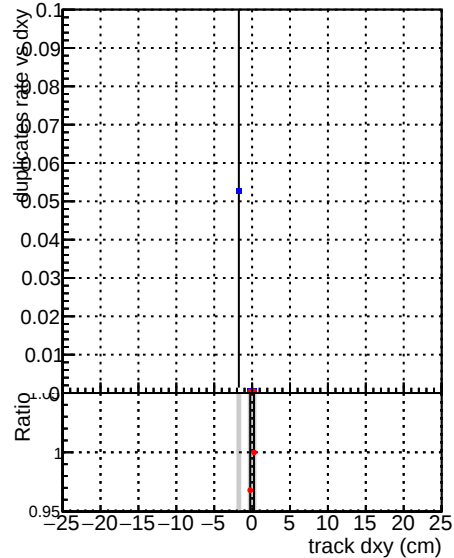
—●— DQM_CKF_TTbase —●— DQM_CKF_TT_retrainOldFiles125_v2_prelimWPM_epoch3
