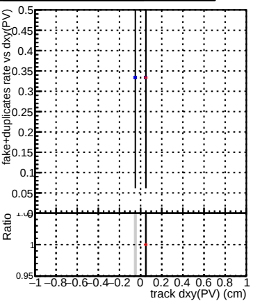
fake+duplicates vs TP dxy(PV)
