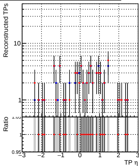
Legend: DQM_CKF_TTbase (blue dots), DQM_CKF_TT_retrainOldFiles125_v2_prelimWPM_epoch3 (red dots)
