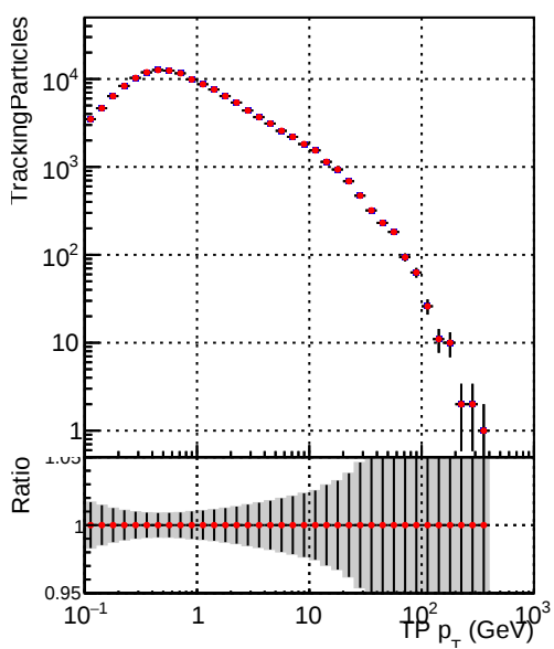
Legend: DQM_CKF_TTbase (blue dots), DQM_CKF_TT_retrainOldFiles125_v2_prelimWPM_epoch3 (red dots)
