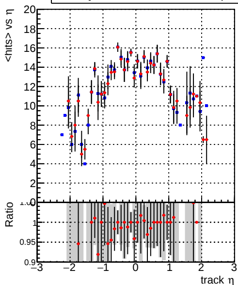
mean hits vs \eta Legend: DQM_CKF_TTbase (blue line with dots), DQM_CKF_TT_retrainOldFiles125_v2_prelimWPM_epoch3 (red line with dots)
