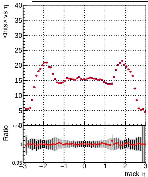
mean hits vs \eta — DQM_CKF_TTbase — DQM_CKF_TT_retrainOldFiles125_v2_prelimWPM_epoch3
