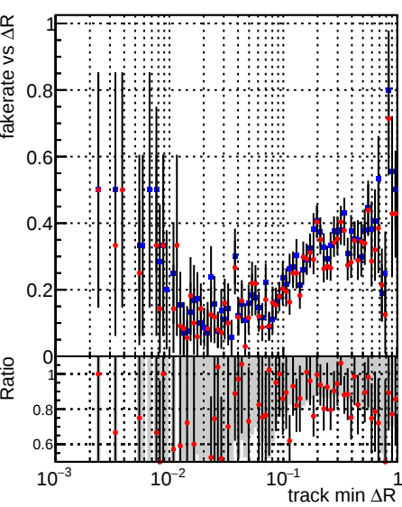
Legend: DQM_CKF_TTbase DQM_CKF_TT_retrainOldFiles125_v2_prelimWPM_epoch3
