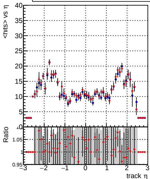
mean hits vs \eta Legend: DQM_CKF_TTbase (blue line with error bars), DQM_CKF_TT_retrainOldFiles125_v2_prelimWPM_epoch3 (red line with error bars)
