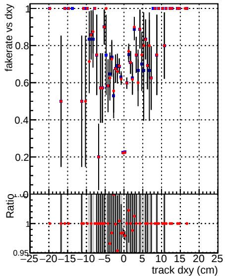
—●— DQM_CKF_TTbase —●— DQM_CKF_TT_retrainOldFiles125_v2_prelimWPM_epoch3
