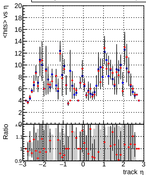
— DQM_CKF_TTbase — DQM_CKF_TT_retrainOldFiles125_v2_prelimWPM_epoch3 mean hits
