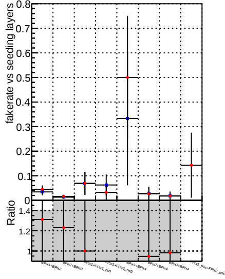
Fake rate vs. DQM_CKF_TTbase DQM_CKF_TT_retrainOldFiles125_v2_prelimWPM_epoch3
