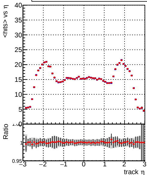
mean hit — DQM_CKF_TTbase — DQM_CKF_TT_retrainOldFiles125_v2_prelimWPM_epoch3
