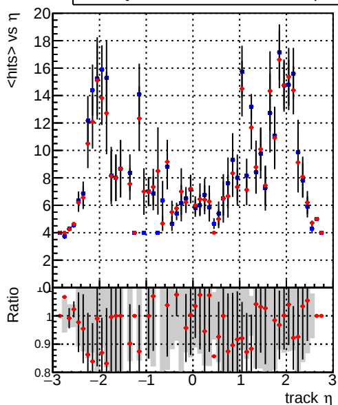
mean hit — DQM_CKF_TTbase — DQM_CKF_TT_retrainOldFiles125_v2_prelimWPM_epoch3
