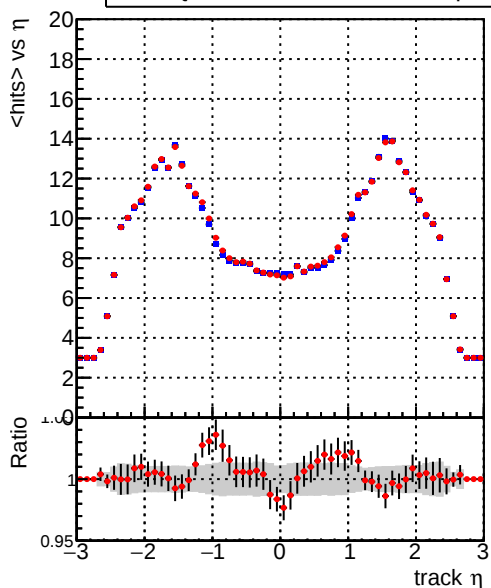
— DQM_CKF_TTbase — DQM_CKF_TT_retrainOldFiles125_v2_prelimWPM_epoch3 mean hits vs \eta
