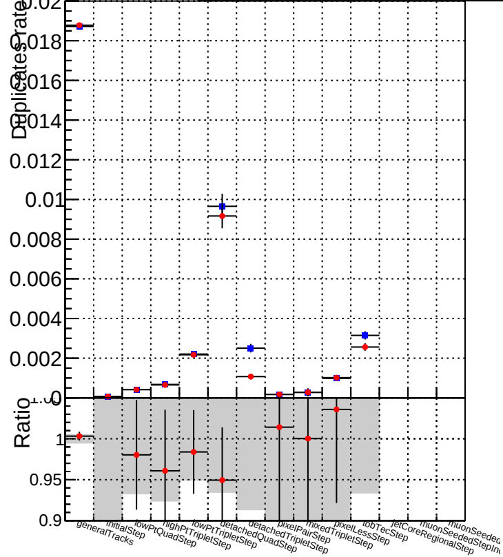
Duplicates rate vs collection Legend: ■ DQM_CKF_TTbase ● DQM_CKF_TT_retrainOldFiles125_v2_prelimWPM_epoch3
