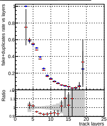
DQM_CKF_TTbase
