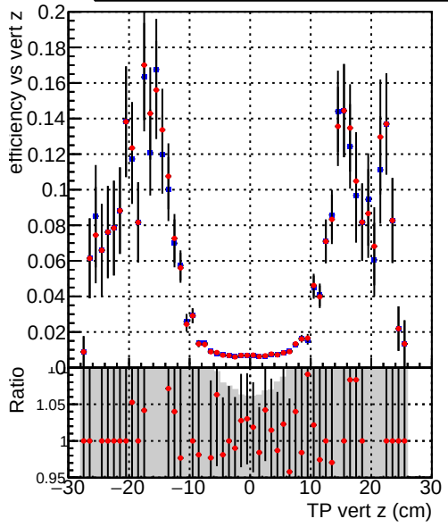
Efficiency vs TP vert z — DQM_CKF_TTbase — DQM_CKF_TT_retrainOldFiles125_v2_prelimWPM_epoch3
